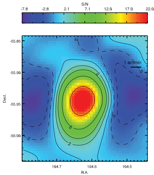
Figure 23. SPT-CL J0658-5556, also known as the Bullet Cluster, RXC J0658.5-5556, and ACT-CL J0658-5557, at z_{\text{spec}} = 0.296 . MPG-ESO/WFI R and V images are shown in the optical/infrared panel. (A color version of this figure is available in the online journal.)
