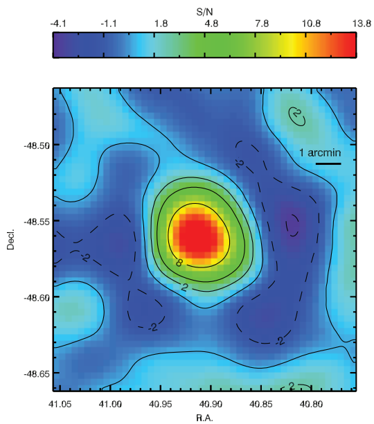
Figure 10. SPT-CL J0243-4833 at z_{\text{rs}} = 0.44 . Blanco/MOSAIC-II irg images are shown in the optical/infrared panel. (A color version of this figure is available in the online journal.)
