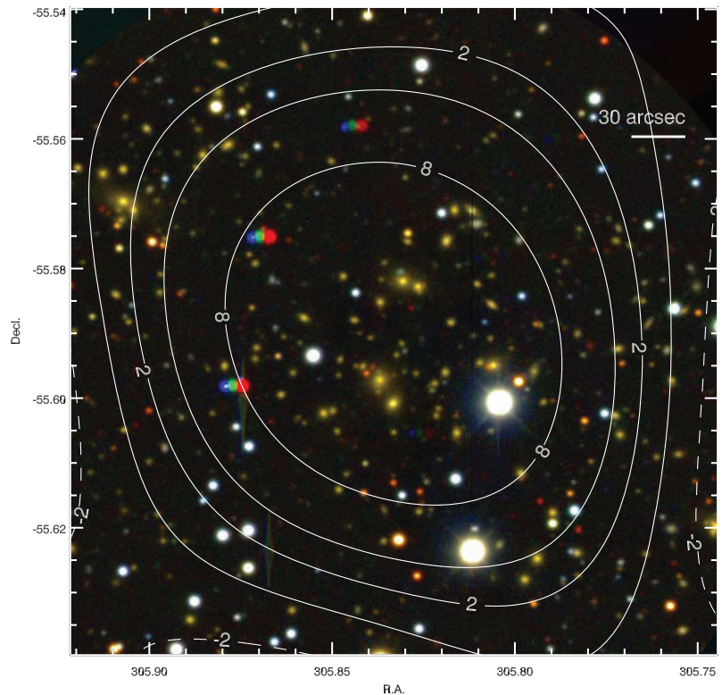
Figure 24. SPT-CL J2023-5535, also known as RXC J2023.4-5535, at z_{\text{spec}} = 0.232 . Magellan/LDSS3 irg images are shown in the optical/infrared panel. (A color version of this figure is available in the online journal.)
