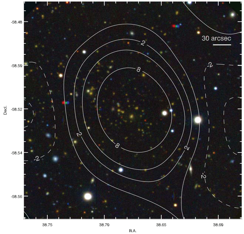
Figure 9. SPT-CL J0234-5831 at z_{\text{spec}} = 0.415 . Magellan/LDSS3 zrg images are shown in the optical/infrared panel. (A color version of this figure is available in the online journal.)
