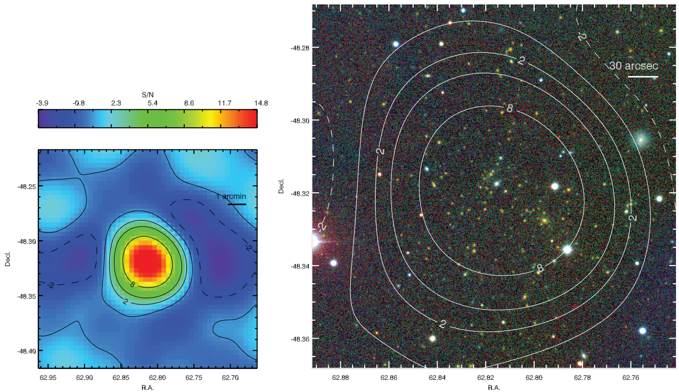
Figure 14. SPT-CL J0411-4819 at z_{rs} = 0.42 . Swope IRV images are shown in the optical/infrared panel. (A color version of this figure is available in the online journal.)
