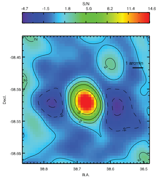
Figure 9. SPT-CL J0234-5831 at z_{\text{spec}} = 0.415 . Magellan/LDSS3 zrg images are shown in the optical/infrared panel. (A color version of this figure is available in the online journal.)
