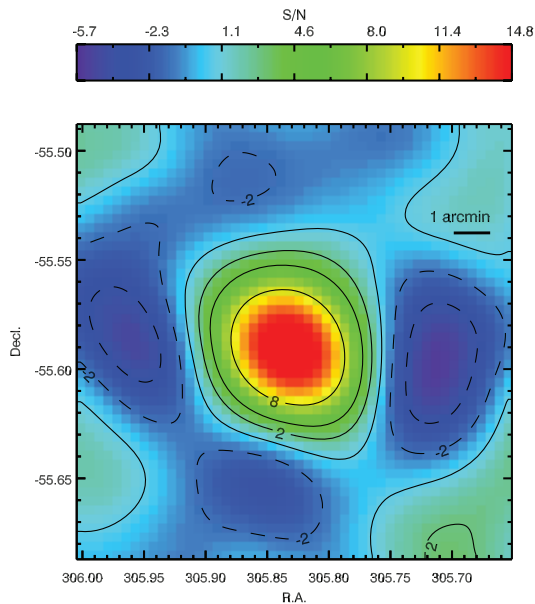
Figure 24. SPT-CL J2023-5535, also known as RXC J2023.4-5535, at z_{\text{spec}} = 0.232 . Magellan/LDSS3 irg images are shown in the optical/infrared panel. (A color version of this figure is available in the online journal.)
