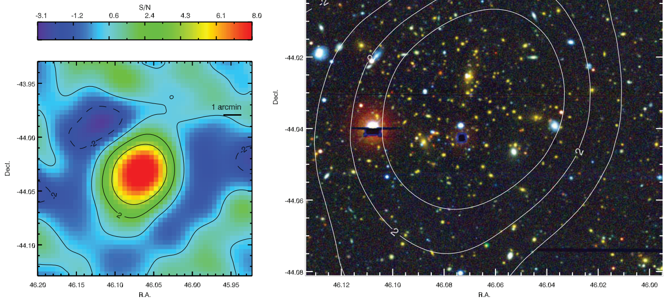
Figure 13. SPT-CL J0304-4401 at z_{rs} = 0.52 . Blanco/MOSAIC-II irg images are shown in the optical/infrared panel. (A color version of this figure is available in the online journal.)
