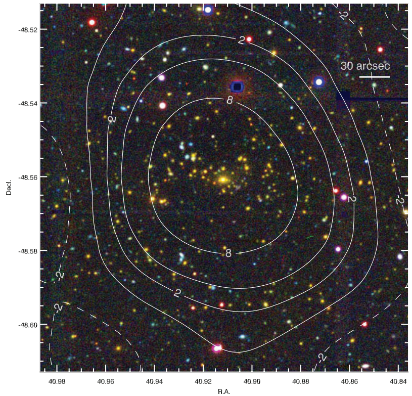
Figure 10. SPT-CL J0243-4833 at z_{\text{rs}} = 0.44 . Blanco/MOSAIC-II irg images are shown in the optical/infrared panel. (A color version of this figure is available in the online journal.)
